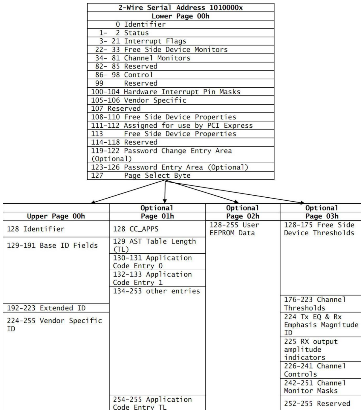
Figure 4, Memory Map
