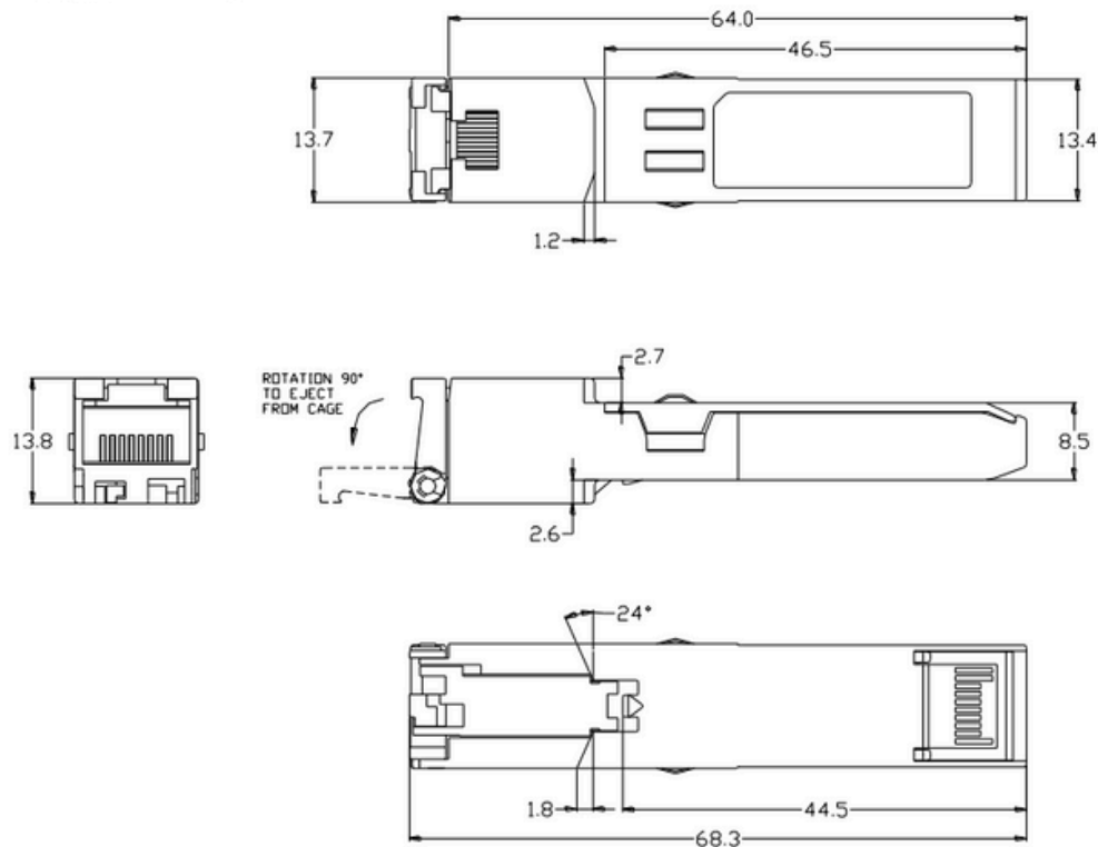
Mechanical Dimensions of Transceiver
